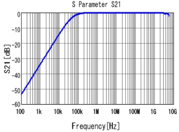
■ GRM31MR72A333KA01 S21 DCOV, 25degC
