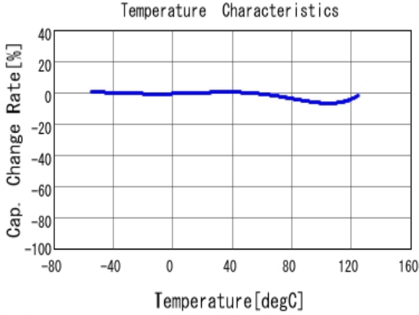
■ GRM31MR72A333KA01 C-Temp. capchange, DCO. 0V, AC1.0V rm
