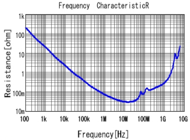
■ GRM31MR72A333KA01 R DCOV, 25degC
