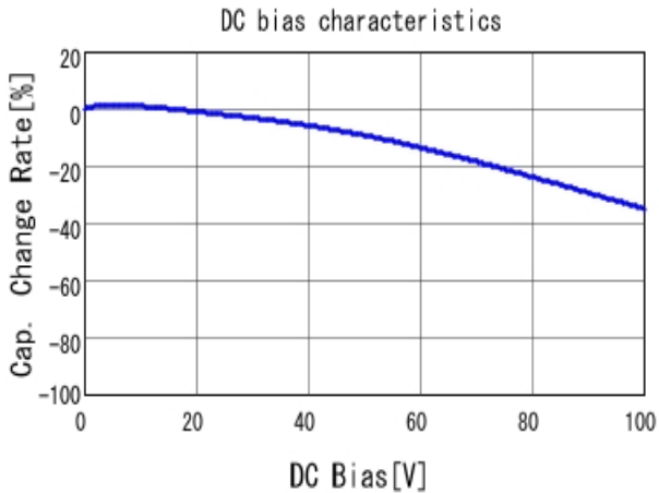
■ GRM31MR72A333KA01 C-DC bias capchange, 25.0degC, AC1.
