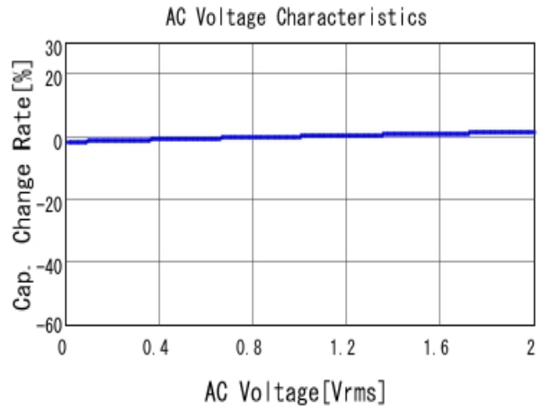
■ GRM31MR72A333KA01 C-AC Voltage capchange, DCOV, 25.0d
