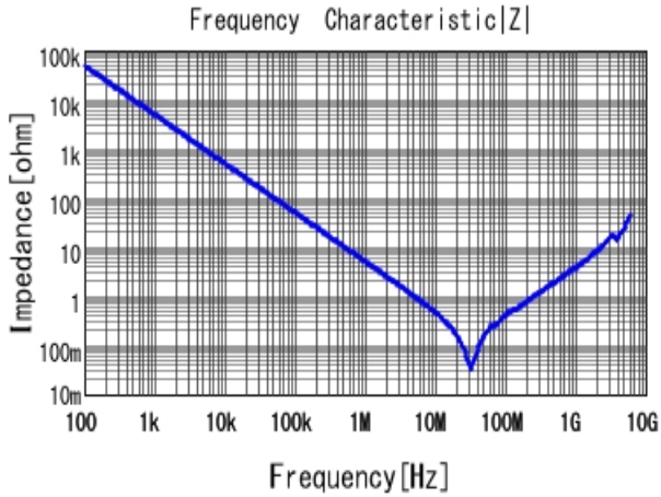
■ GRM31MR72A333KA01 |Z| DCOV, 25degC
