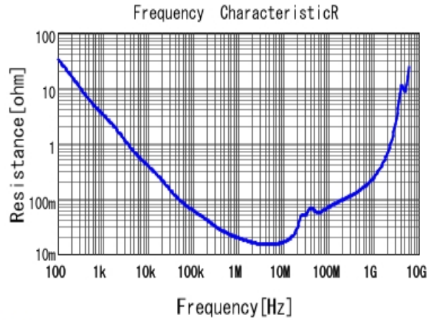
■ GRM31MR72A224KA01 R DCOV, 25degC
