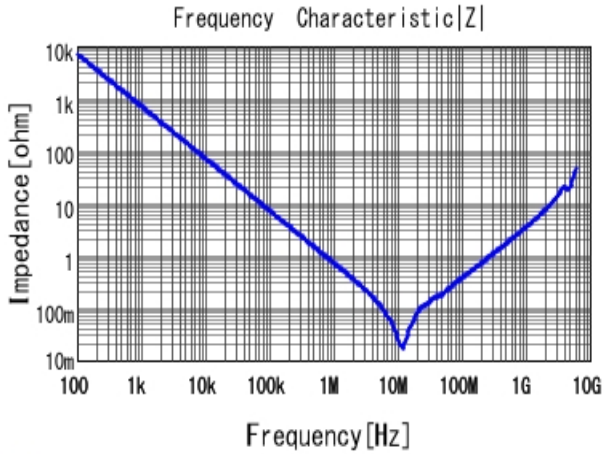
■ GRM31MR72A224KA01 |Z| DCOV, 25degC
