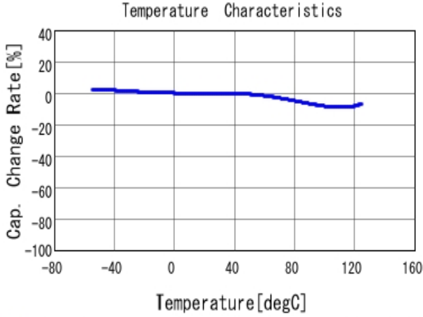
■ GRM31MR72A224KA01 C-Temp. capchange, DC0.0V, AC1.0V r m
