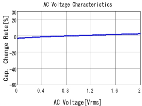
■ GRM31MR72A224KA01 C-AC Voltage capchange, DCOV, 25.0d
