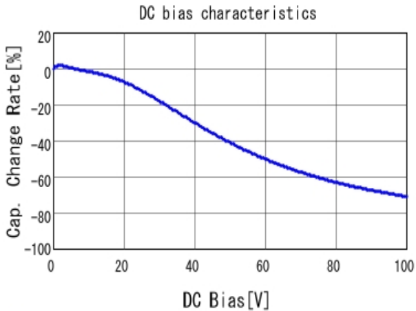
■ GRM31MR72A224KA01 C-DC bias capchange, 25.0degC, AC1.
