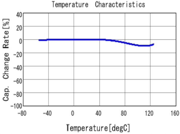
■ GRM31MR72A223KA01 C-Temp. capchange, DCO. 0V, AC1.0Vrm
