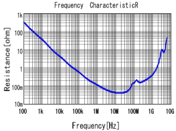
■ GRM31MR72A223KA01 R DCOV, 25degC
