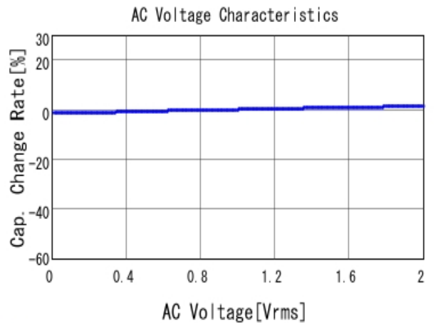
■ GRM31MR72A223KA01 C-AC Voltage capchange, DCOV, 25.0d
