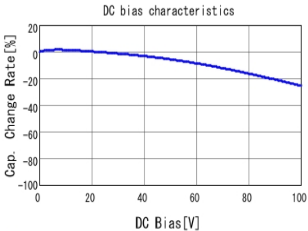
■ GRM31MR72A223KA01 C-DC bias capchange, 25.0degC, AC1.
