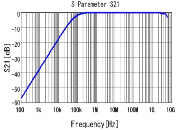
■ GRM31MR72A223KA01 S21 DCOV, 25degC
