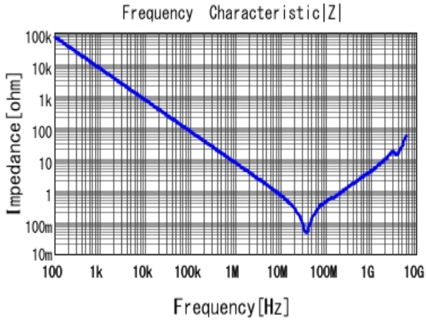
■ GRM31MR72A223KA01 |Z| DCOV, 25degC
