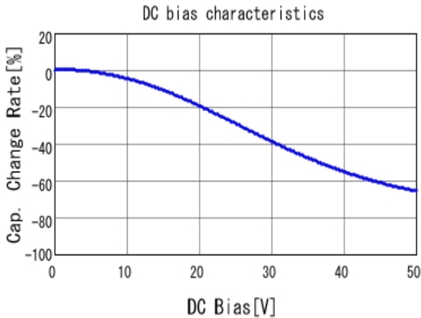
■ GRM31MR71H684KA88 C-DC bias capchange, 25.0degC, AC1.
