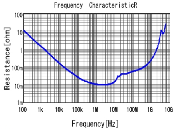
■ GRM31MR71H684KA88 R DCOV, 25degC
