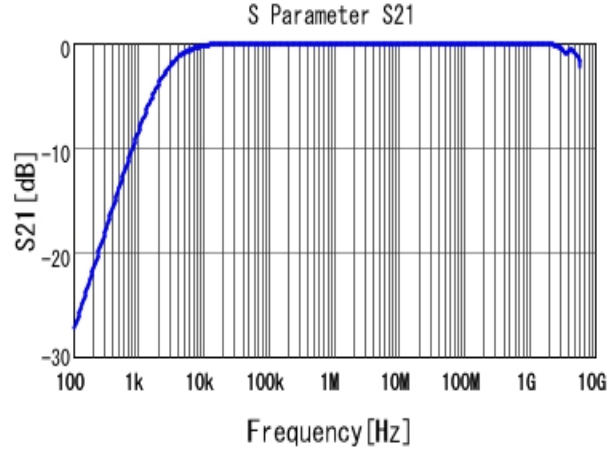
■ GRM31MR71H684KA88 S21 DCOV, 25degC
