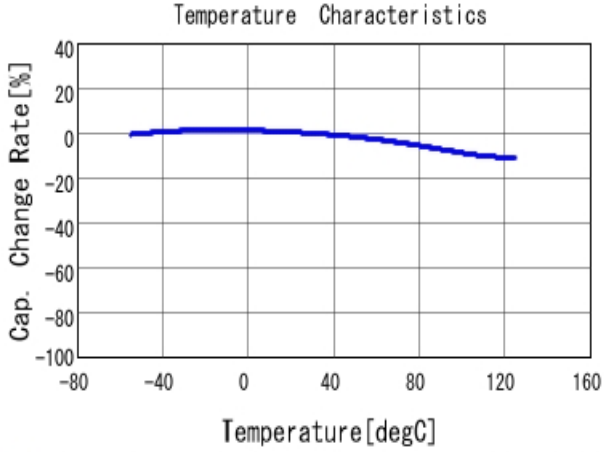
■ GRM31MR71H684KA88 C-Temp. capchange, DCO. 0V, AC1.0V rm
