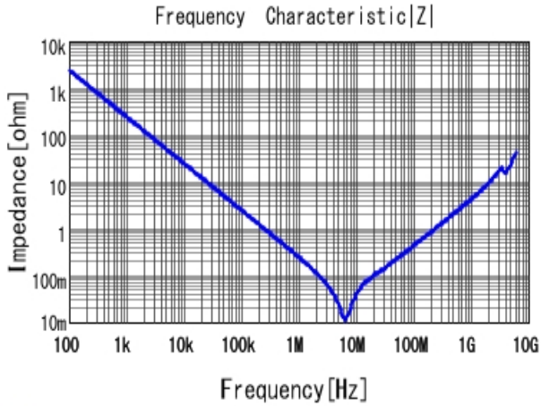
■ GRM31MR71H684KA88 |Z| DCOV, 25degC
