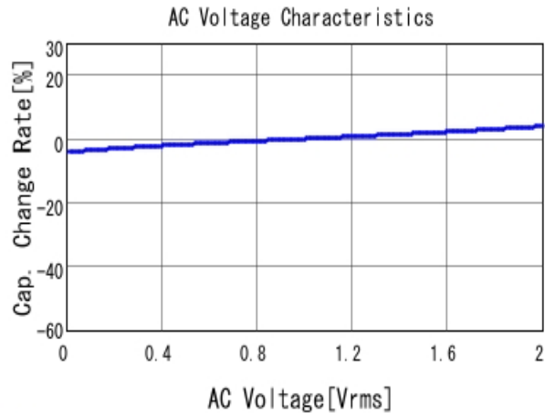
■ GRM31MR71H684KA88 C-AC Voltage capchange, DCOV, 25.0d
