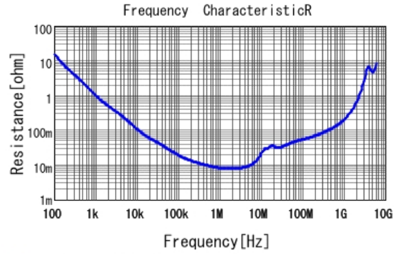
■ GRM31MR71H105KA88 R DCOV, 25degC
