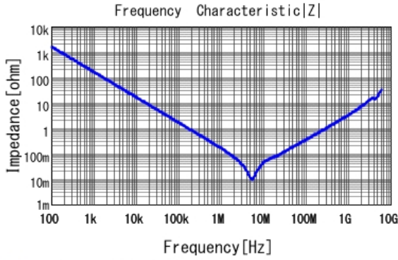
■ GRM31MR71H105KA88 |Z| DCOV, 25degC
