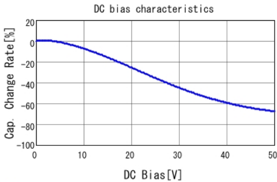
■ GRM31MR71H105KA88 C-DC bias capchange, 25.0degC, AC1.
