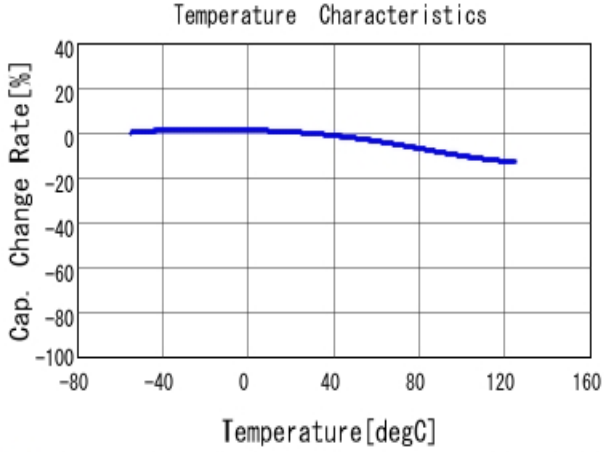
■ GRM31MR71E225KA93 C-Temp. capchange, DC0.0V, AC1.0V r m
