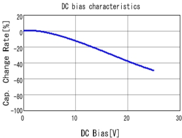
■ GRM31MR71E225KA93 C-DC bias capchange, 25.0degC, AC1.
