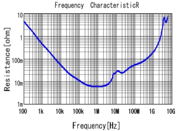
■ GRM31MR71E225KA93 R DCOV, 25degC
