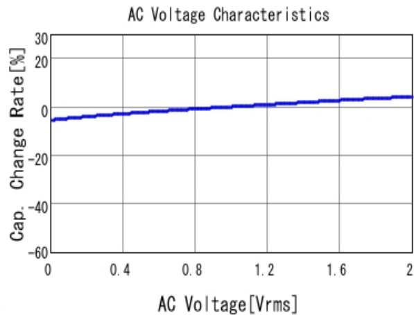
■ GRM31MR71E225KA93 C-AC Voltage capchange, DCOV, 25.0d
