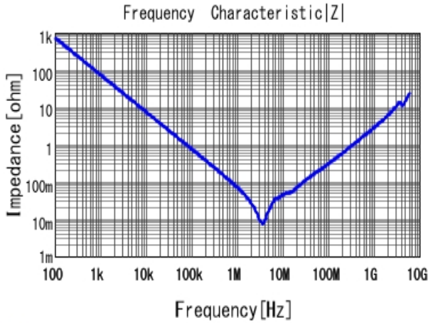
■ GRM31MR71E225KA93 |Z| DCOV, 25degC
