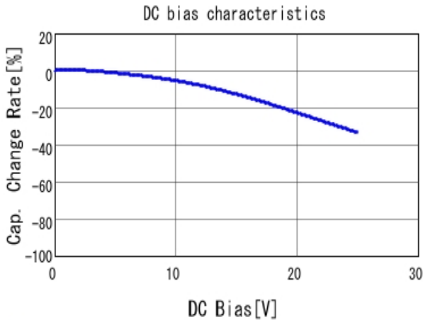
■ GRM31MR71E105KA01 C-DC bias capchange, 25.0degC, AC1.
