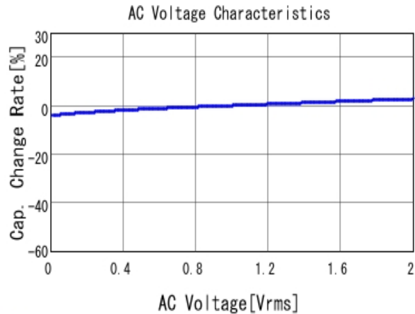
■ GRM31MR71E105KA01 C-AC Voltage capchange, DCOV, 25.0d
