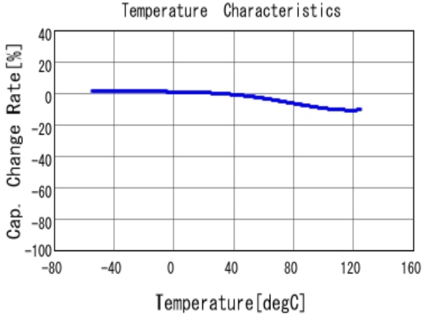
■ GRM31MR71E105KA01 C-Temp. capchange, DC0.0V, AC1.0V rm
