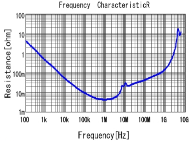
■ GRM31MR71C225KA35 R DCOV, 25degC
