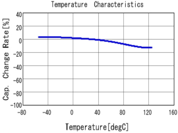
■ GRM31MR71C225KA35 C-Temp. capchange, DC0.0V, AC1.0V r m
