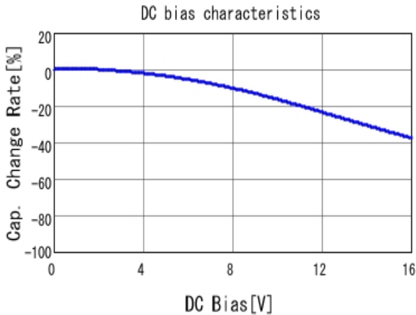
■ GRM31MR71C225KA35 C-DC bias capchange, 25.0degC, AC1.
