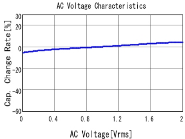
■ GRM31MR71C225KA35 C-AC Voltage capchange, DCOV, 25.0d
