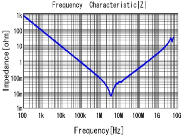
■ GRM31MR71C225KA35 |Z| DCOV, 25degC
