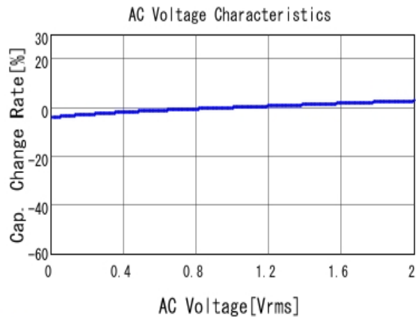
■ GRM31MR71C105KA01 C-AC Voltage capchange, DCOV, 25.0d
