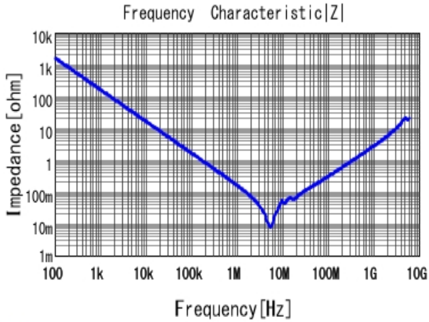
■ GRM31MR71C105KA01 |Z| DCOV, 25degC
