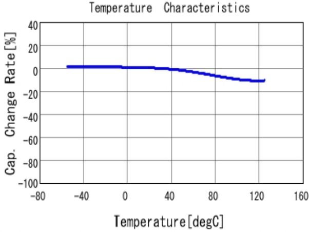
■ GRM31MR71C105KA01 C-Temp. capchange, DC0.0V, AC1.0V rm
