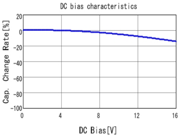
■ GRM31MR71C105KA01 C-DC bias capchange, 25.0degC, AC1.
