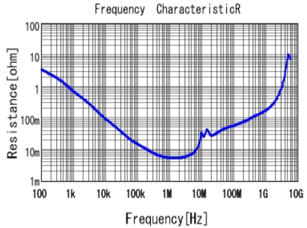
■ GRM31MR71C105KA01 R DCOV, 25degC
