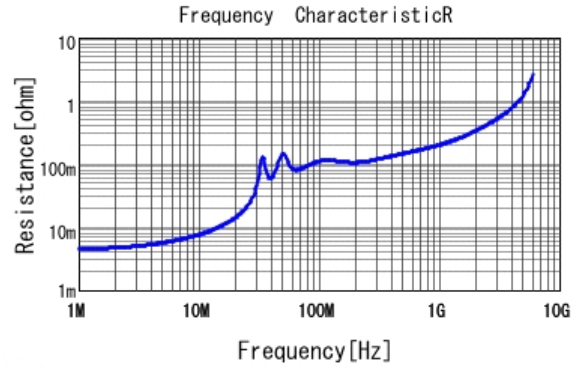
■ GRM31M7U1H104JA01 R DC0V, 25degC
