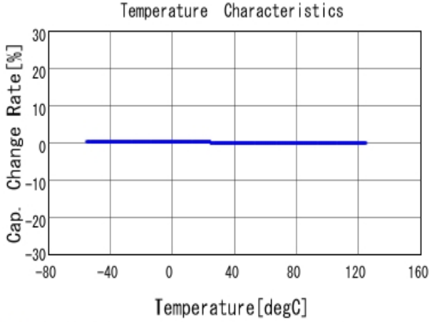
■ GRM31M5C1H473JA01 C-Temp. capchange, DCOV, AC1Vrms
