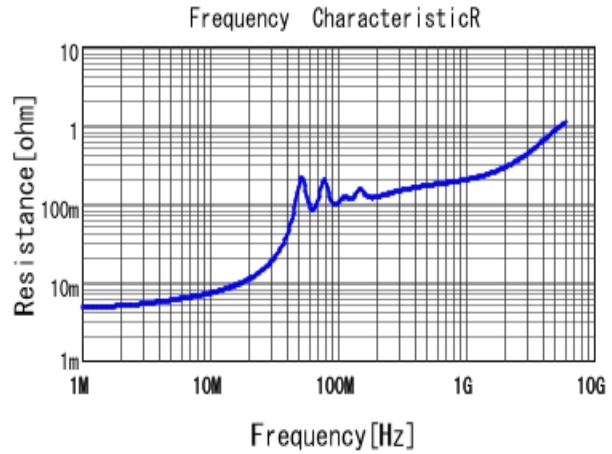
■ GRM31M5C1H473JA01 R DCOV, 25degC
