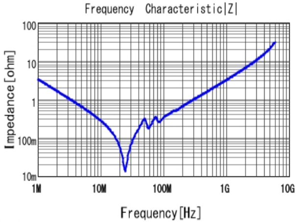
■ GRM31M5C1H473JA01 |Z| DCOV, 25degC
