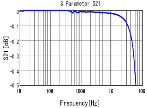
■ GRM31M5C1H473JA01 S21 DCOV, 25degC
