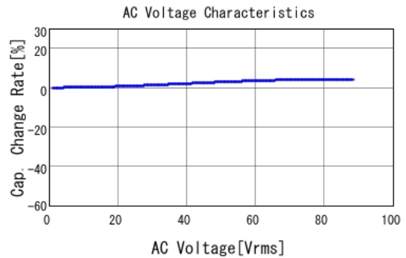
■ GRM31CR72E473KW03 C-AC Voltage capchange, DCOV, 25.0d
