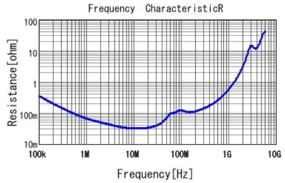
■ GRM31CR72E473KW03 R DCOV, 25degC
