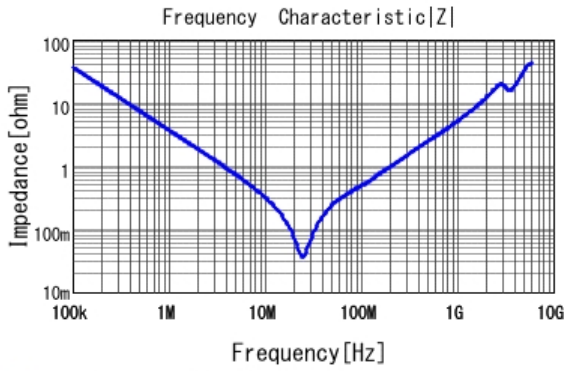
■ GRM31CR72E473KW03 |Z| DCOV, 25degC
