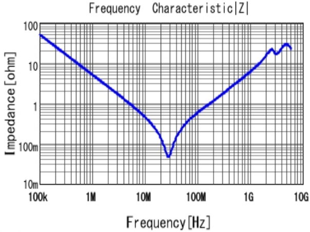
■ GRM31CR72E333KW03 |Z| DCOV, 25degC
