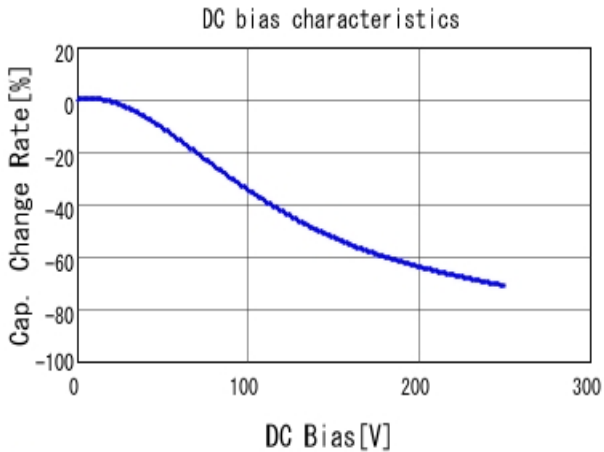
■ GRM31CR72E333KW03 C-DC bias capchange, 25.0degC, AC1V
