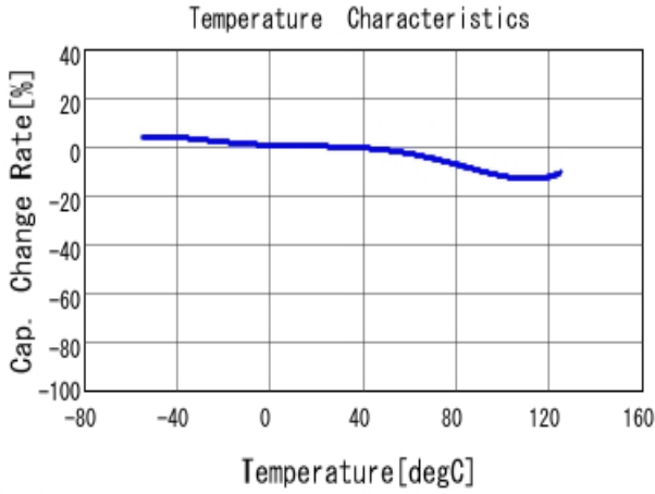
■ GRM31CR72E333KW03 C-Temp. capchange, DCOV, AC1Vrms
