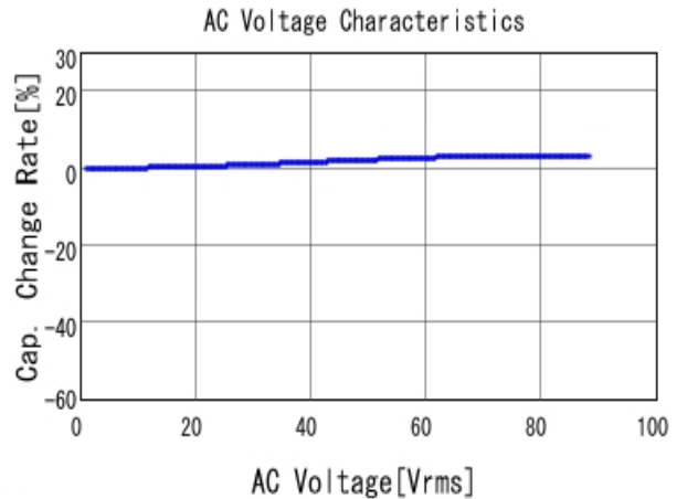
■ GRM31CR72E333KW03 C-AC Voltage capchange, DCOV, 25.0d
