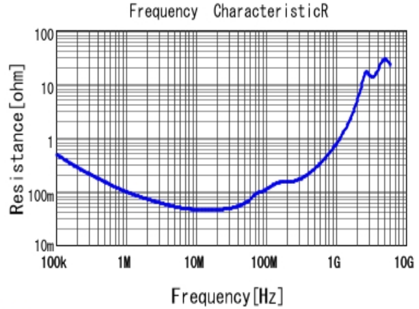
■ GRM31CR72E333KW03 R DCOV, 25degC
