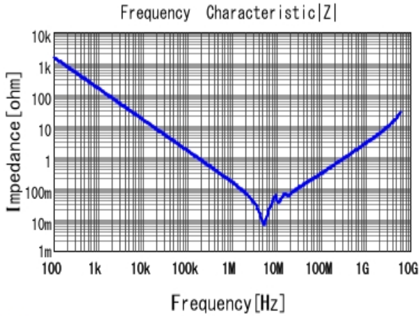
■ GRM31CR72A105KA01 |Z| DCOV, 25degC
