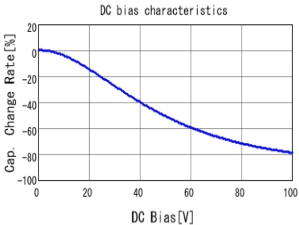
■ GRM31CR72A105KA01 C-DC bias capchange, 25.0degC, AC1.
