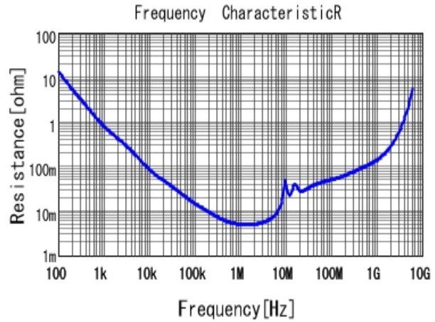
■ GRM31CR72A105KA01 R DCOV, 25degC
