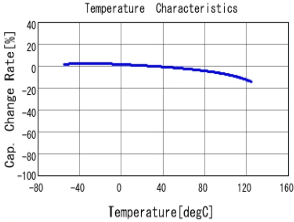
■ GRM31CR72A105KA01 C-Temp. capchange, DC0.0V, AC1.0V r m
