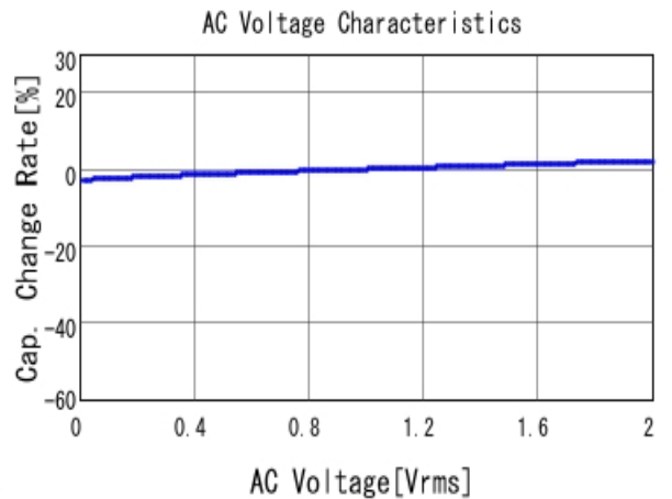
■ GRM31CR72A105KA01 C-AC Voltage capchange, DCOV, 25.0d
