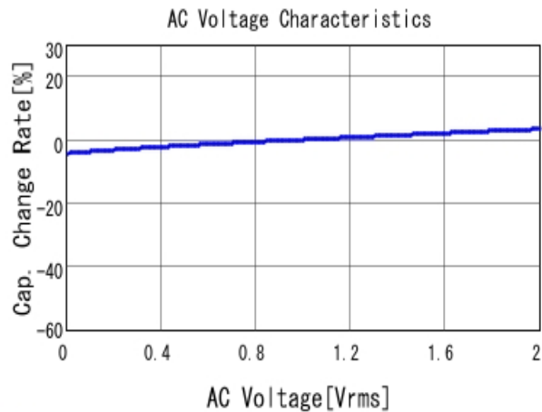
■ GRM31CR71H225KA88 C-AC Voltage capchange, DCOV, 25.0d
