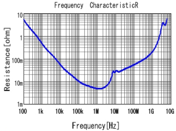
■ GRM31CR71H225KA88 R DCOV, 25degC
