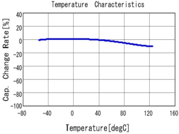
■ GRM31CR71H225KA88 C-Temp. capchange, DC0.0V, AC1.0V rm
