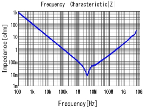
■ GRM31CR71H225KA88 |Z| DCOV, 25degC
