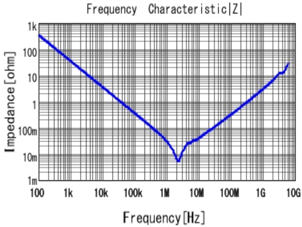
■ GRM31CR71E475KA88 |Z| DCOV, 25degC
