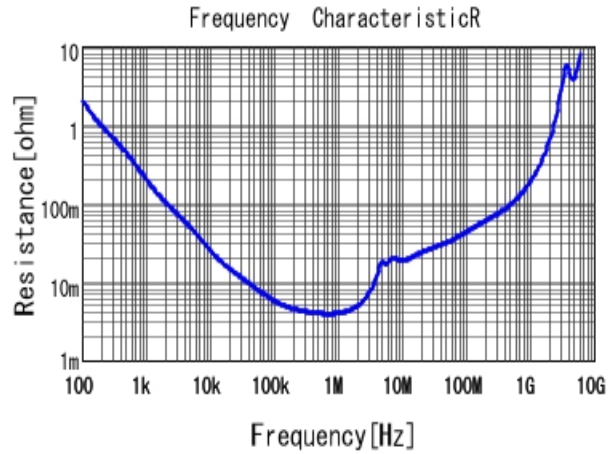
■ GRM31CR71E475KA88 R DCOV, 25degC
