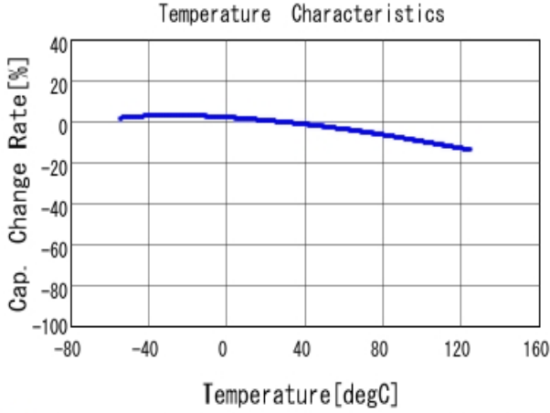
■ GRM31CR71E475KA88 C-Temp. capchange, DC0.0V, AC1.0V rm
