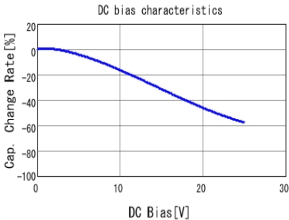
■ GRM31CR71E475KA88 C-DC bias capchange, 25.0degC, AC1.
