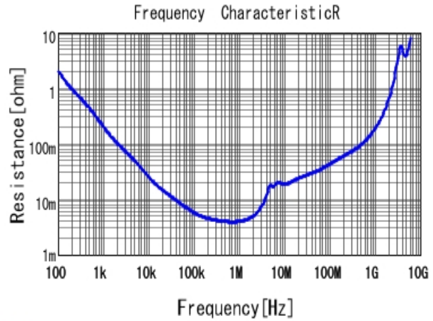
■ GRM31CR71C475KA01 R DCOV, 25degC
