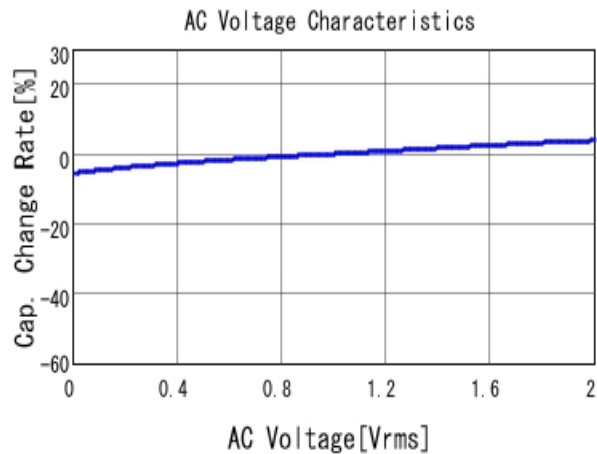
■ GRM31CR71C475KA01 C-AC Voltage capchange, DCOV, 25.0d
