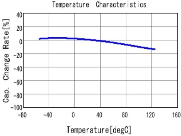
■ GRM31CR71C475KA01 C-Temp. capchange, DC0.0V, AC1.0V rm
