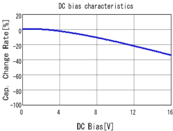
■ GRM31CR71C475KA01 C-DC bias capchange, 25.0degC, AC1.
