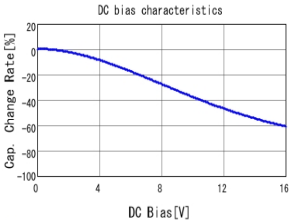
■ GRM31CR71C106KAC7 C-DC bias capchange, 25.0degC, AC1.
