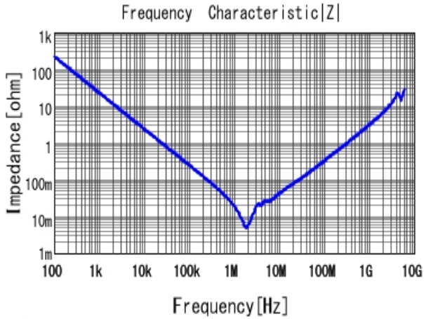
■ GRM31CR71C106KAC7 |Z| DCOV, 25degC
