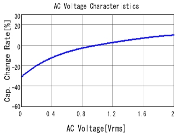
■ GRM31CR71C106KAC7 C-AC Voltage capchange, DCOV, 25.0d
