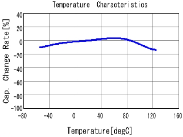
■ GRM31CR71C106KAC7 C-Temp. capchange, DC0.0V, AC1.0V r m
