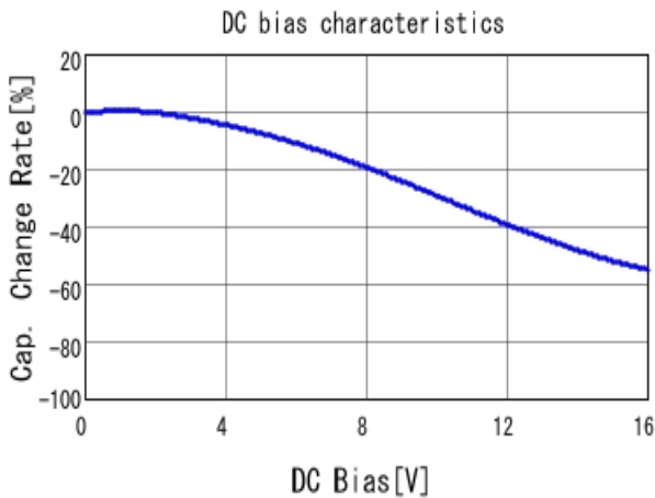
■ GRM31CR71C106KA12 C-DC bias capchange, 25.0degC, AC1.
