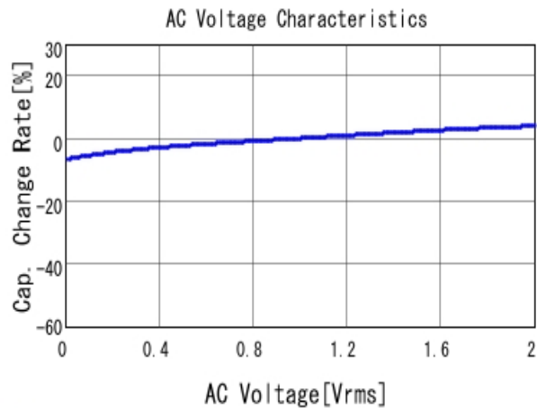
■ GRM31CR71C106KA12 C-AC Voltage capchange, DCOV, 25.0d
