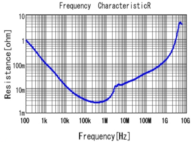
■ GRM31CR71C106KA12 R DCOV, 25degC
