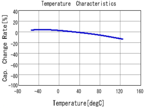
■ GRM31CR71C106KA12 C-Temp. capchange, DCO. 0V, AC1.0V rm
