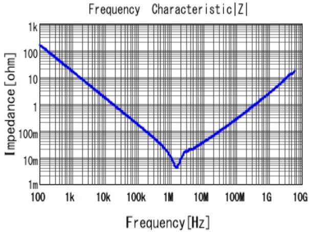
■ GRM31CR71C106KA12 |Z| DCOV, 25degC
