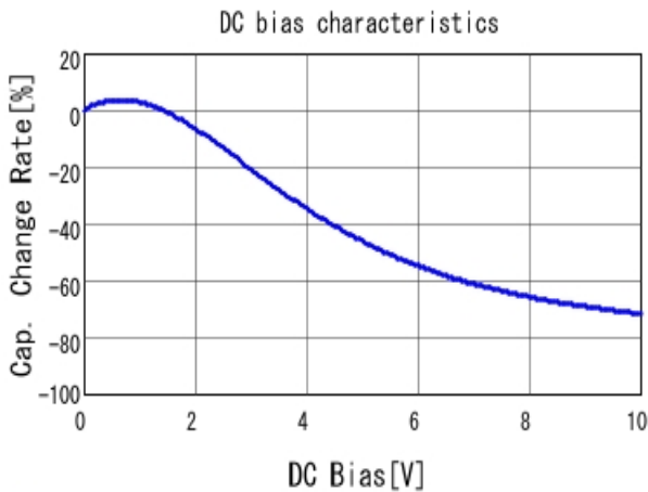
■ GRM31CR71A226KE15 C-DC bias capchange, 25.0degC, AC0.
