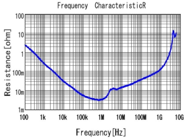
■ GRM31CR71A226KE15 R DCOV, 25degC
