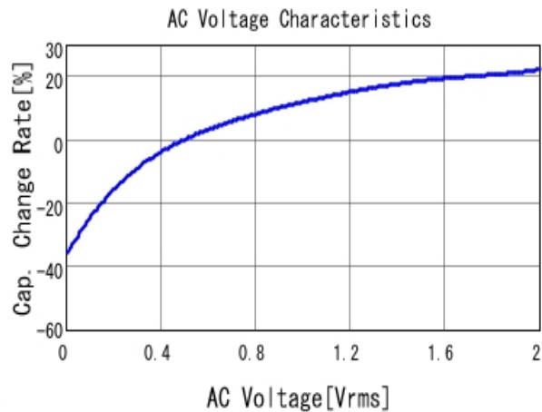
■ GRM31CR71A226KE15 C-AC Voltage capchange, DCOV, 25.0d
