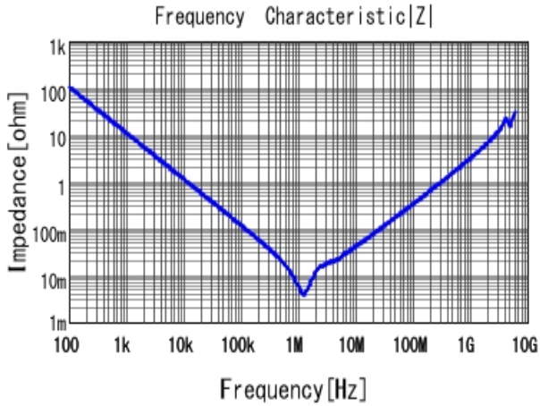
■ GRM31CR71A226KE15 |Z| DCOV, 25degC
