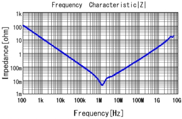
■ GRM31CR70J226ME19 |Z| DCOV, 25degC
