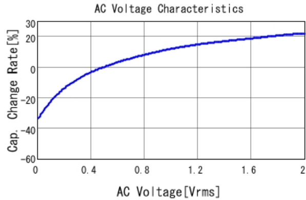
■ GRM31CR70J226ME19 C-AC Voltage capchange, DCOV, 25.0d
