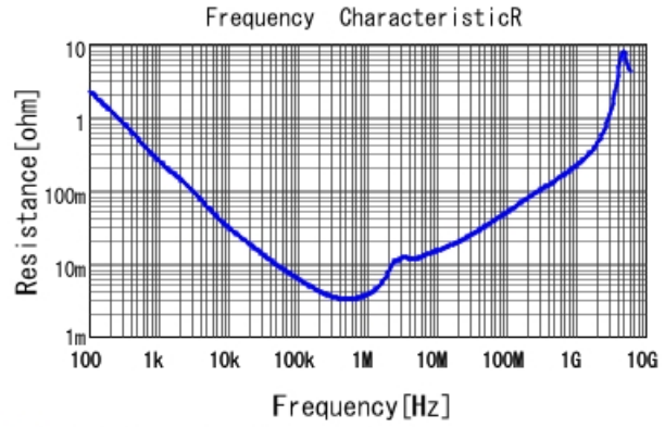
■ GRM31CR70J226ME19 R DCOV, 25degC
