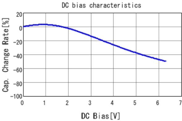
■ GRM31CR70J226ME19 C-DC bias capchange, 25.0degC, AC0.
