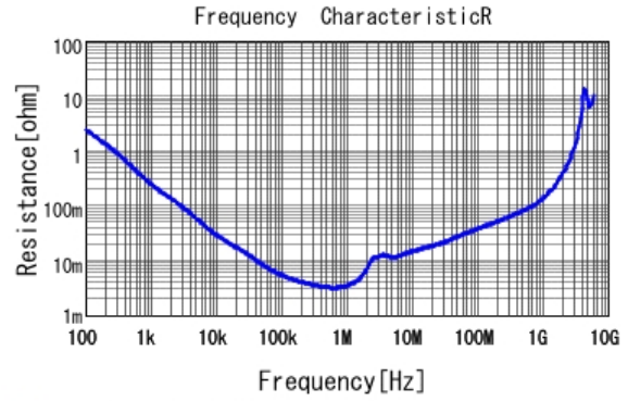
■ GRM31CR70J226KE19 R DCOV, 25degC
