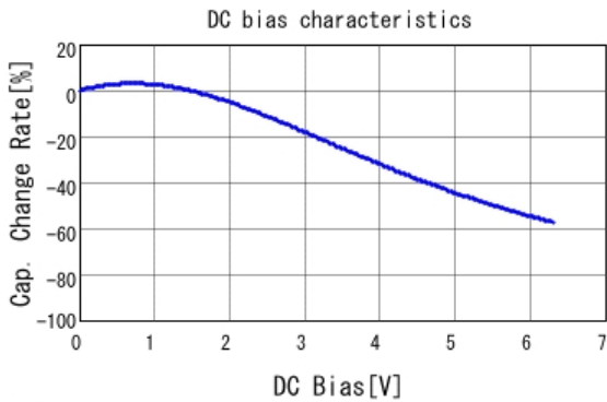
■ GRM31CR70J226KE19 C-DC bias capchange, 25.0degC, AC0.
