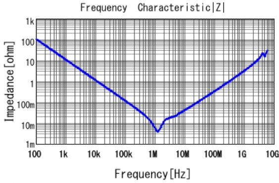
■ GRM31CR70J226KE19 |Z| DCOV, 25degC
