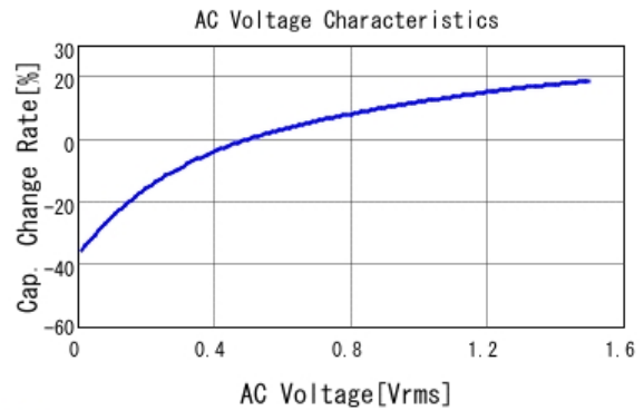
■ GRM31CR70J226KE19 C-AC Voltage capchange, DCOV, 25.0d
