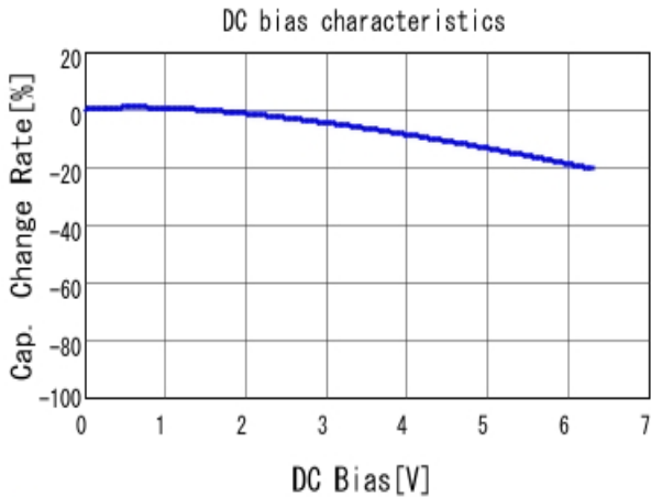
■ GRM31CR70J106KA01 C-DC bias capchange, 25.0degC, AC1.
