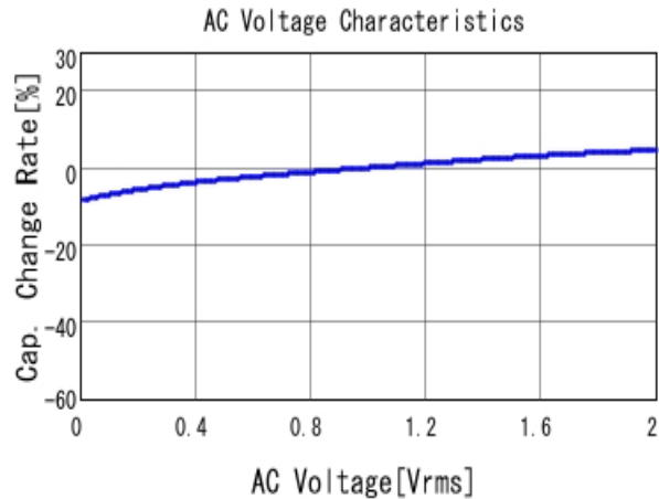
■ GRM31CR70J106KA01 C-AC Voltage capchange, DCOV, 25.0d
