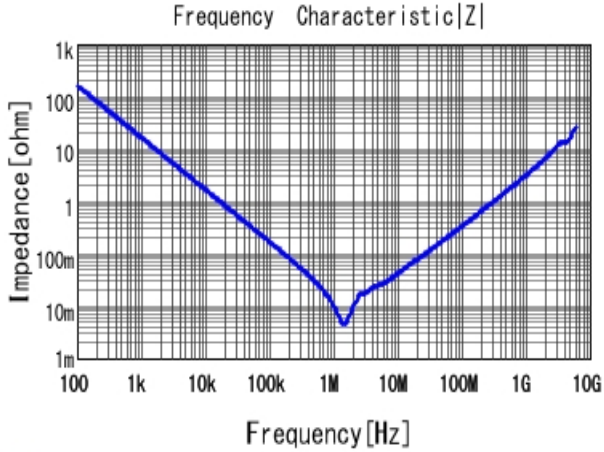
■ GRM31CR70J106KA01 |Z| DCOV, 25degC
