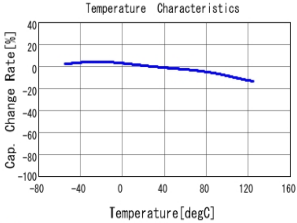
■ GRM31CR70J106KA01 C-Temp. capchange, DC0.0V, AC1.0V r m
