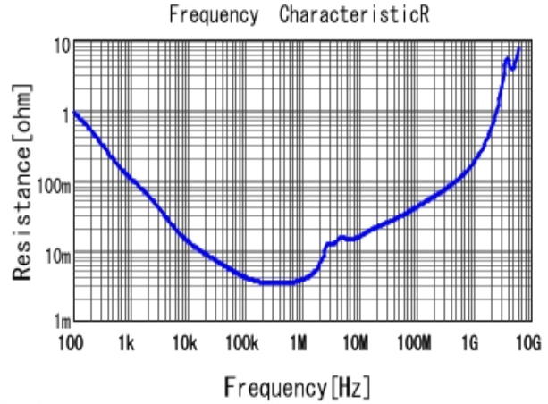
■ GRM31CR70J106KA01 R DCOV, 25degC
