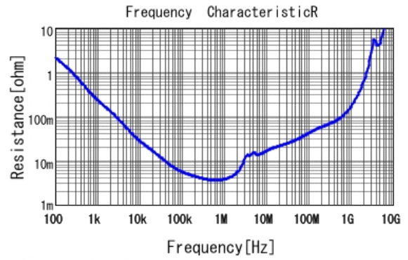
■ GRM31CR6YA106KA12 R DCOV, 25degC
