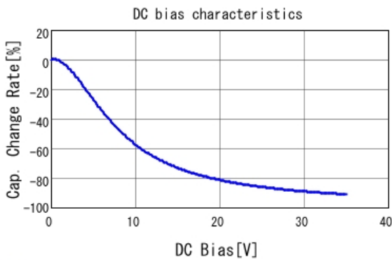
■ GRM31CR6YA106KA12 C-DC bias capchange, 25.0degC, AC1.
