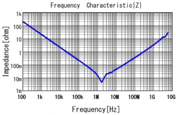
■ GRM31CR6YA106KA12 |Z| DCOV, 25degC
