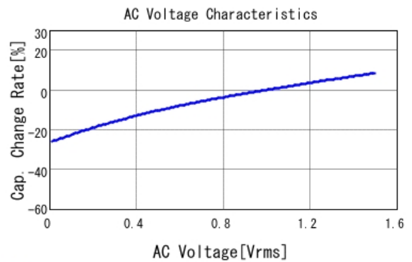
■ GRM31CR6YA106KA12 C-AC Voltage capchange, DCOV, 25.0d
