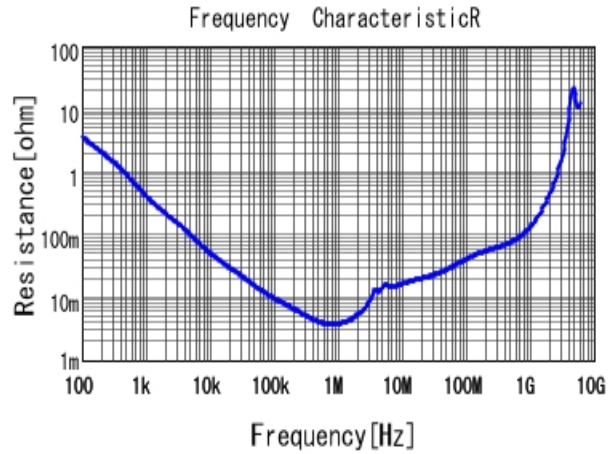
■ GRM31CR61H106KA12 R DCOV, 25degC
