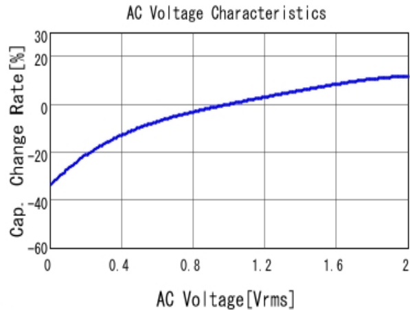
■ GRM31CR61H106KA12 C-AC Voltage capchange, DCOV, 25.0d
