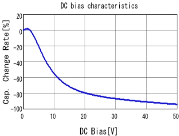
■ GRM31CR61H106KA12 C-DC bias capchange, 25.0degC, AC1.
