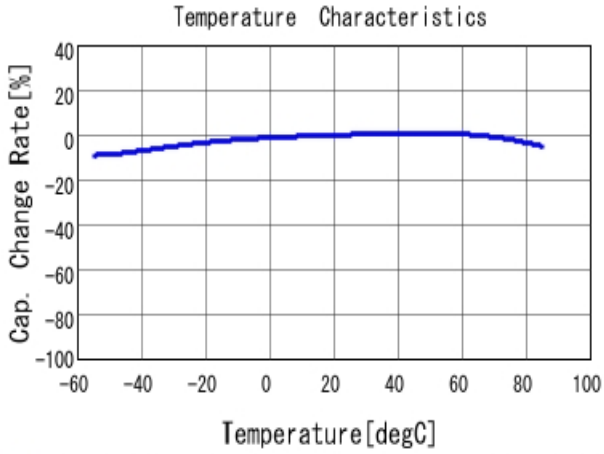
■ GRM31CR61H106KA12 C-Temp. capchange, DC0.0V, AC1.0V rm
