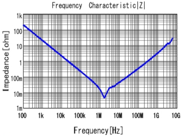
■ GRM31CR61E106KA12 |Z| DCOV, 25degC
