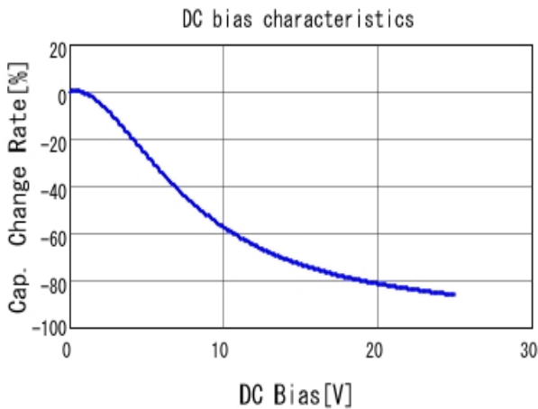
■ GRM31CR61E106KA12 C-DC bias capchange, 25.0degC, AC1.
