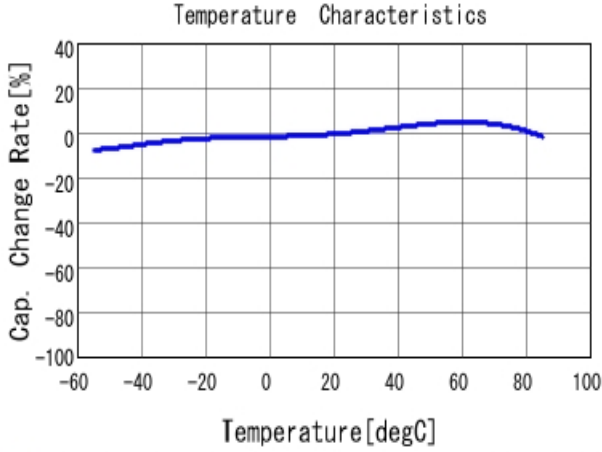
■ GRM31CR61E106KA12 C-Temp. capchange, DC0.0V, AC1.0V r m
