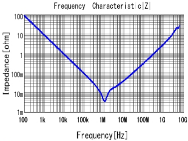
■ GRM31CR61C226KE15 |Z| DCOV, 25degC
