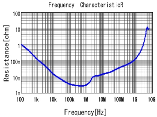
■ GRM31CR61C226KE15 R DCOV, 25degC
