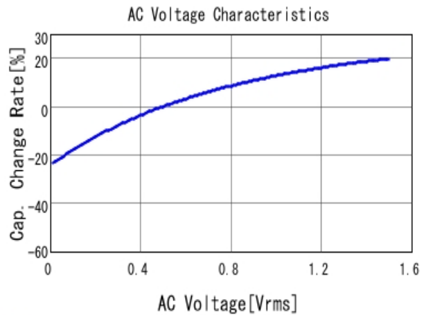
■ GRM31CR61C226KE15 C-AC Voltage capchange, DCOV, 25.0d
