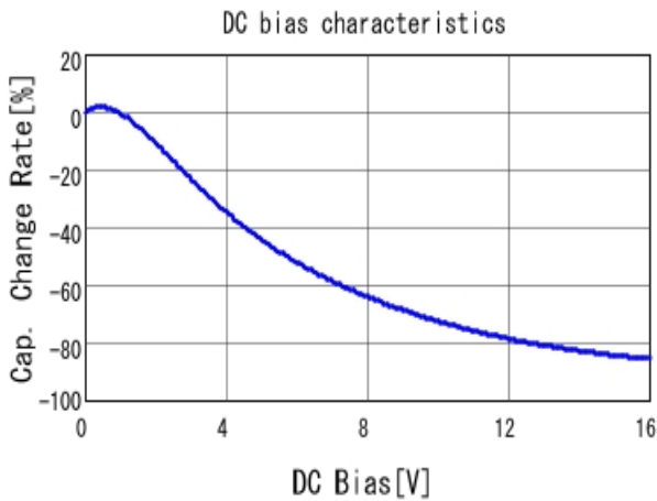
■ GRM31CR61C226KE15 C-DC bias capchange, 25.0degC, AC0.
