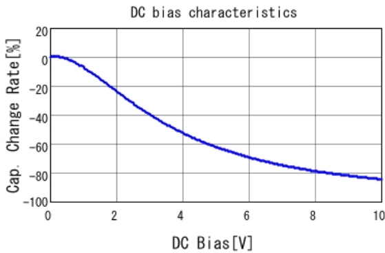
■ GRM31CR61A476KE15 C-DC bias capchange, 25.0degC, AC0.
