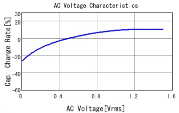
■ GRM31CR61A476KE15 C-AC Voltage capchange, DCOV, 25.0d
