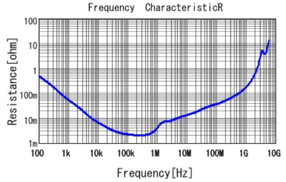
■ GRM31CR61A476KE15 R DCOV, 25degC
