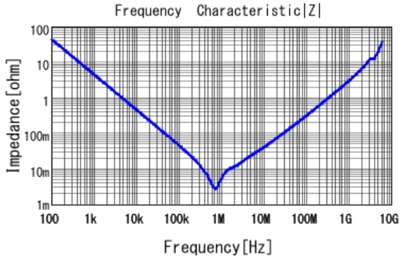
■ GRM31CR61A476KE15 |Z| DCOV, 25degC
