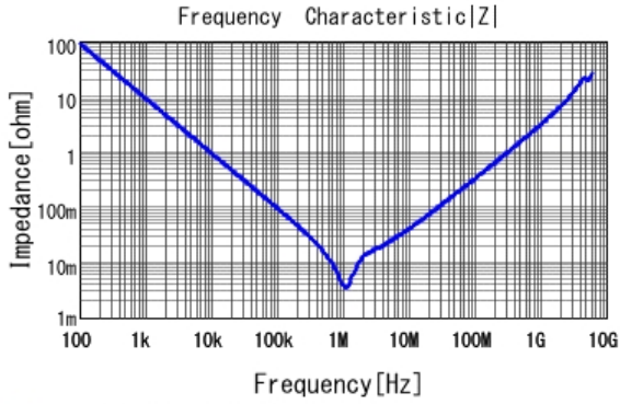
■ GRM31CR61A226ME19 |Z| DCOV, 25degC
