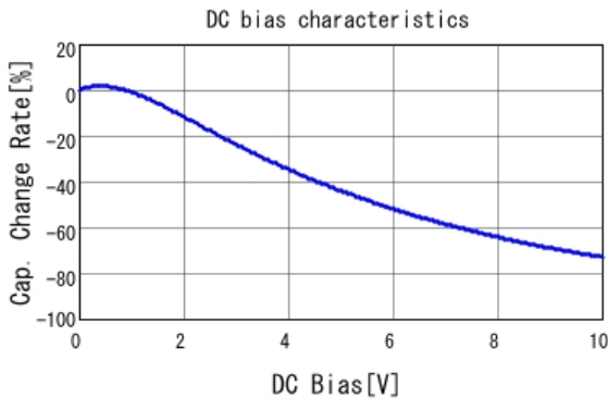
■ GRM31CR61A226ME19 C-DC bias capchange, 25.0degC, AC0.
