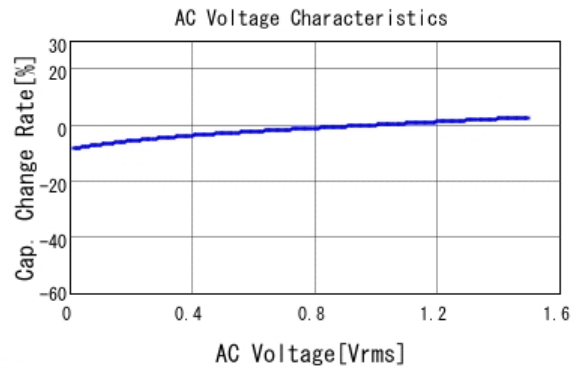
■ GRM31CR61A106KA01 C-AC Voltage capchange, DCOV, 25.0d
