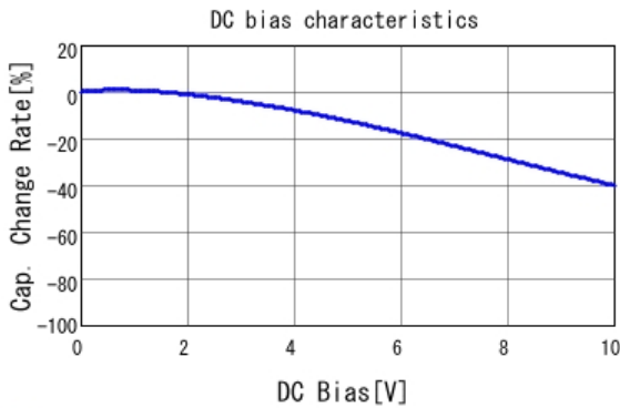
■ GRM31CR61A106KA01 C-DC bias capchange, 25.0degC, AC1.
