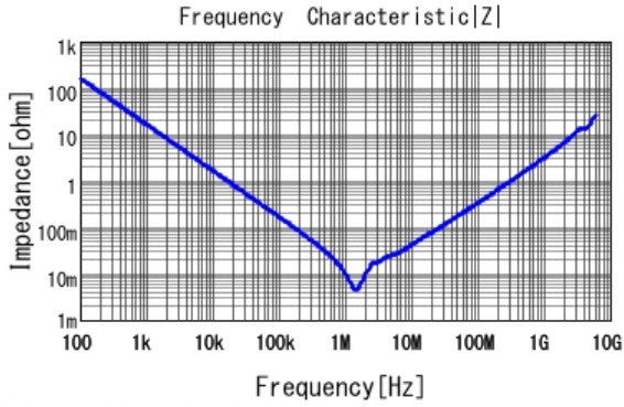
■ GRM31CR61A106KA01 |Z| DCOV, 25degC
