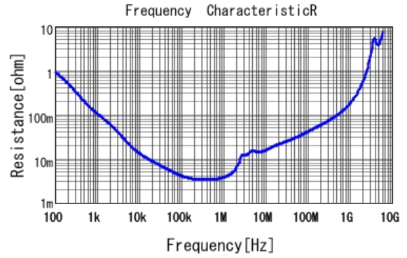
■ GRM31CR61A106KA01 R DCOV, 25degC
