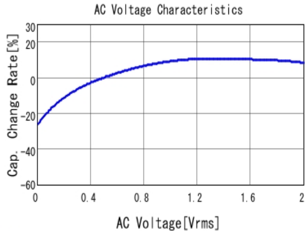
■ GRM31CR60J476ME19 C-AC Voltage capchange, DCOV, 25.0d
