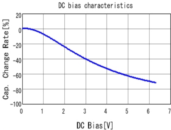
■ GRM31CR60J476ME19 C-DC bias capchange, 25.0degC, AC0.
