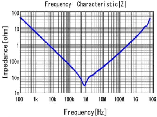
■ GRM31CR60J476ME19 |Z| DCOV, 25degC
