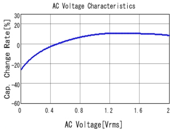
■ GRM31CR60J476KE19 C-AC Voltage capchange, DCOV, 25.0d
