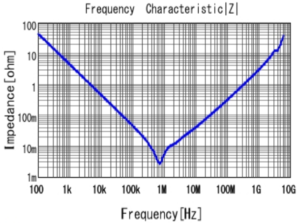
■ GRM31CR60J476KE19 |Z| DCOV, 25degC
