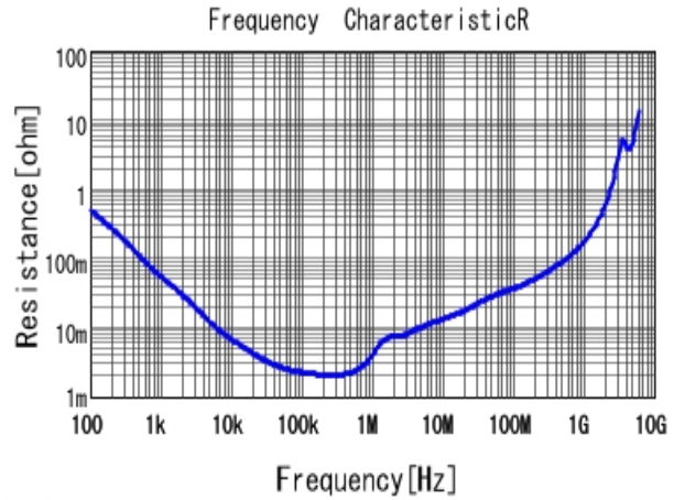
■ GRM31CR60J476KE19 R DCOV, 25degC
