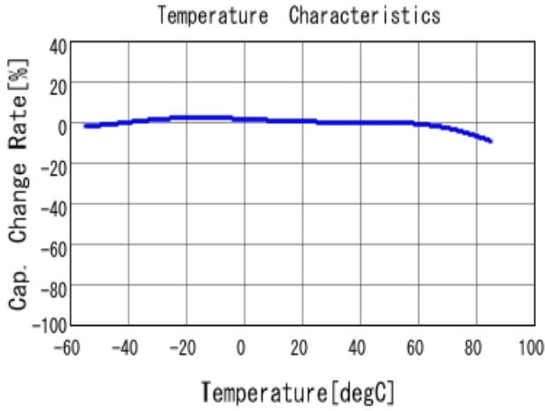
■ GRM31CR60J476KE19 C-Temp. capchange, DCO. 0V, ACO. 5V rm
