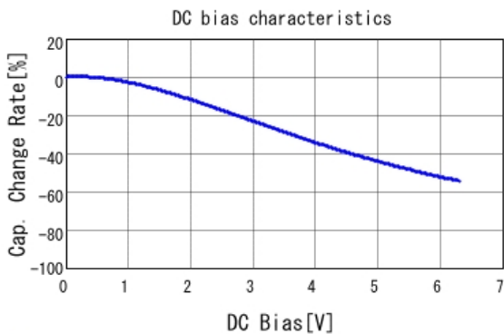
■ GRM31CR60J226KE19 C-DC bias capchange, 25.0degC, ACO.
