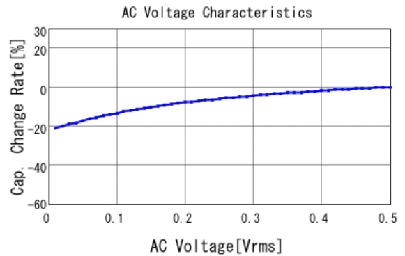
■ GRM31CR60G227ME11 C-AC Voltage capchange, DCOV, 25.0d
