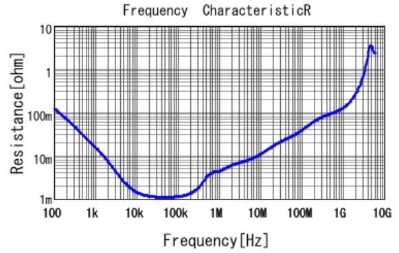
■ GRM31CR60G227ME11 R DCOV, 25degC
