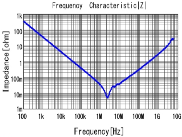
■ GRM31CC72A475KE11 |Z| DCOV, 25degC
