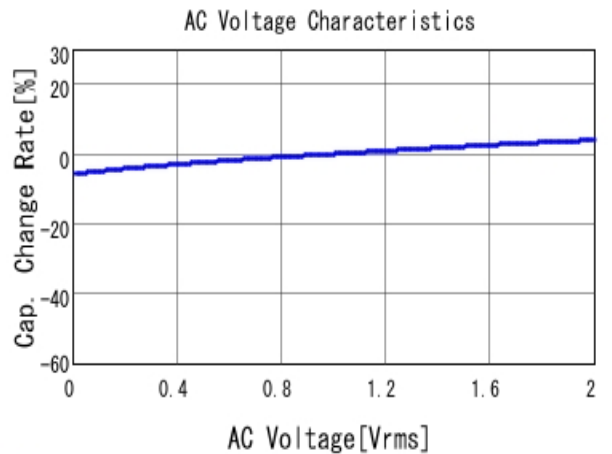
■ GRM31CC72A475KE11 C-AC Voltage capchange, DCOV, 25.0d
