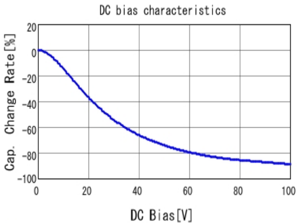
■ GRM31CC72A475KE11 C-DC bias capchange, 25.0degC, AC1V
