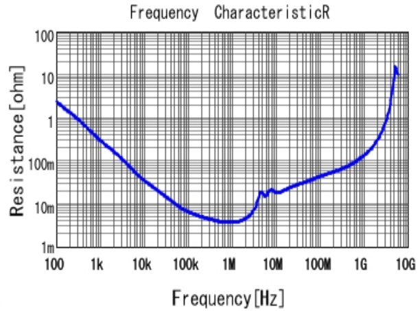
■ GRM31CC72A475KE11 R DCOV, 25degC
