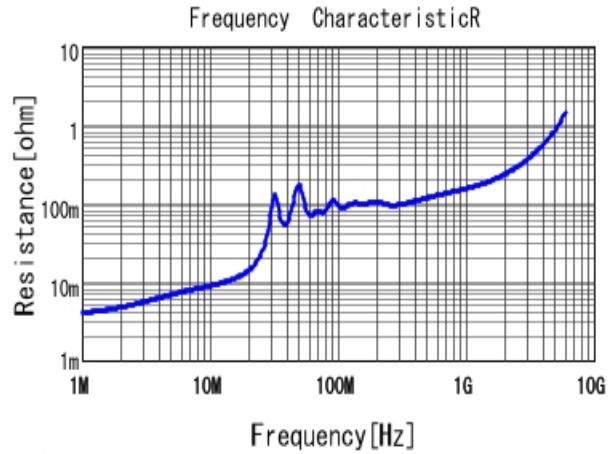
■ GRM31C5C2A104JA01 R DCOV, 25degC
