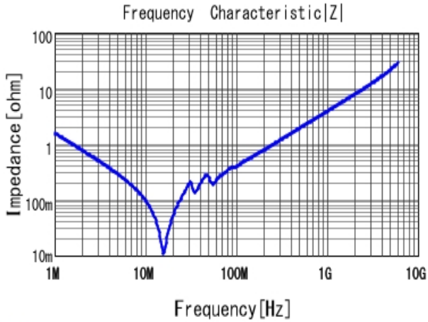
■ GRM31C5C2A104JA01 |Z| DCOV, 25degC
