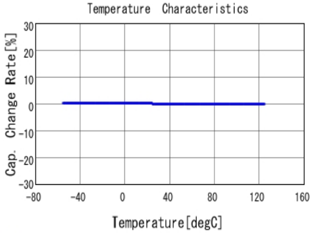
■ GRM31C5C1H823JA01 C-Temp. capchange, DCOV, AC1Vrms
