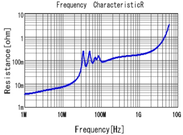
■ GRM31C5C1H823JA01 R DCOV, 25degC
