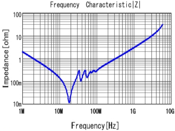
■ GRM31C5C1H823JA01 |Z| DCOV, 25degC
