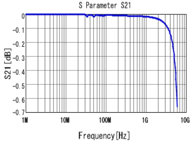
■ GRM31C5C1H823JA01 S21 DCOV, 25degC
