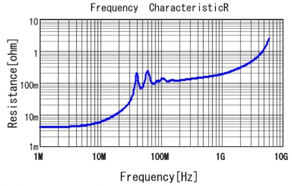
■ GRM31C5C1H683JA01 R DCOV, 25degC
