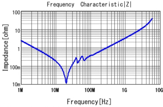
■ GRM31C5C1H683JA01 |Z| DCOV, 25degC
