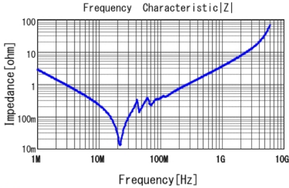
■ GRM31C5C1H563JA01 |Z| DCOV, 25degC
