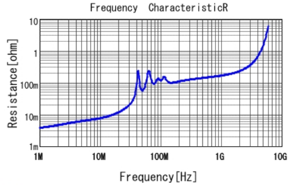
■ GRM31C5C1H563JA01 R DCOV, 25degC
