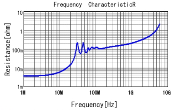
■ GRM31C5C1H104JA01 R DCOV, 25degC
