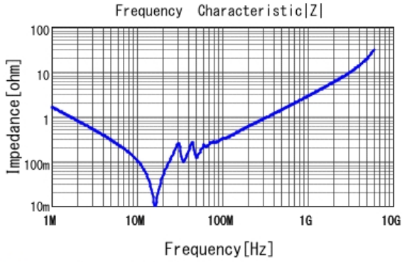
■ GRM31C5C1H104JA01 |Z| DCOV, 25degC
