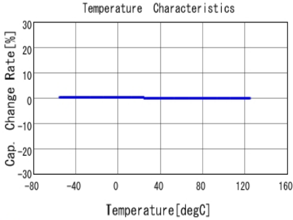
■ GRM31C5C1E104JA01 C-Temp. capchange, DCOV, AC1Vrms
