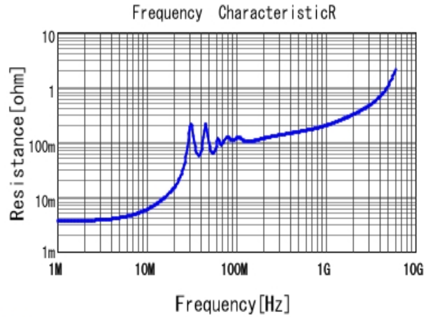
■ GRM31C5C1E104JA01 R DCOV, 25degC
