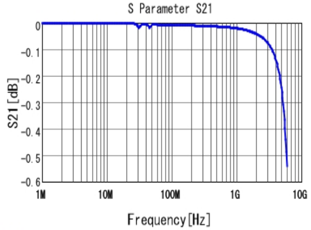
■ GRM31C5C1E104JA01 S21 DCOV, 25degC
