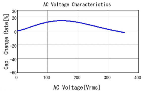
■ GRM31BR73A471KW01 C-AC Voltage capchange, DCOV, 25.0d
