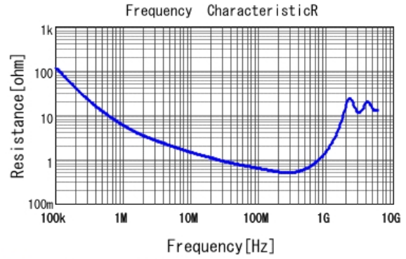
■ GRM31BR73A471KW01 R DCOV, 25degC
