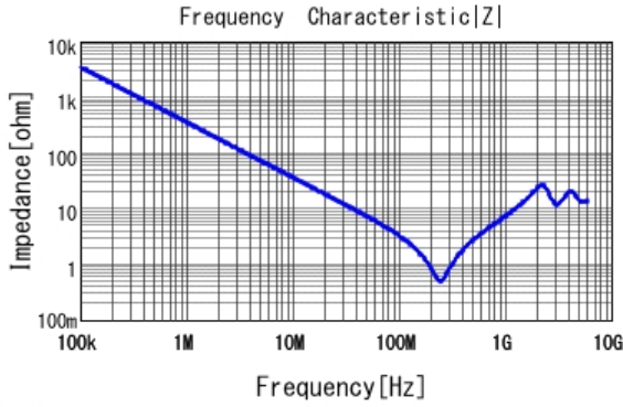
■ GRM31BR73A471KW01 |Z| DCOV, 25degC
