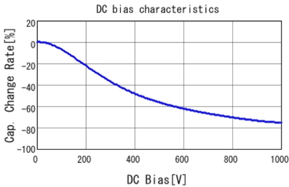
■ GRM31BR73A471KW01 C-DC bias capchange, 25.0degC, AC1V
