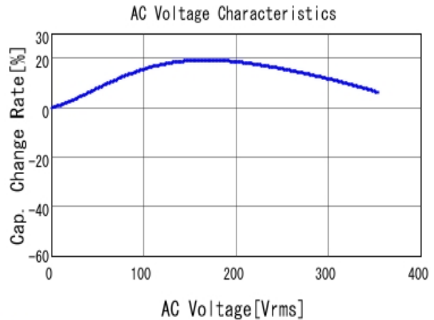
■ GRM31BR73A152KW01 C-AC Voltage capchange, DCOV, 25.0d
