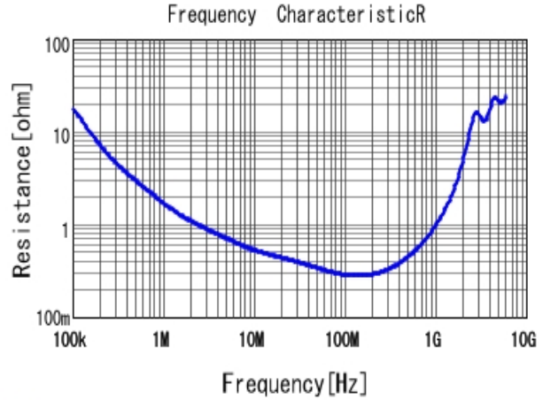
■ GRM31BR73A152KW01 R DCOV, 25degC
