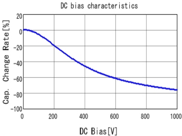
■ GRM31BR73A152KW01 C-DC bias capchange, 25.0degC, AC1V
