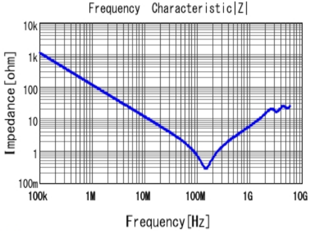
■ GRM31BR73A152KW01 |Z| DCOV, 25degC
