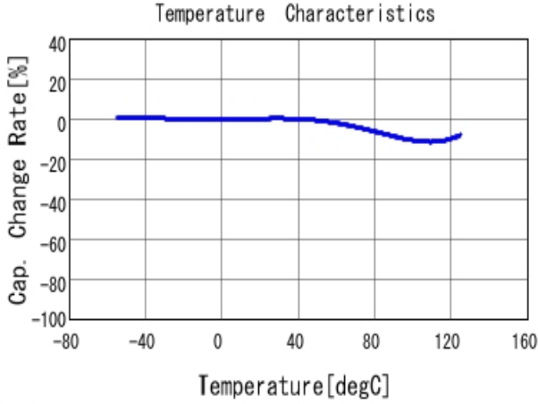
■ GRM31BR73A102KW01 C-Temp. capchange, DCOV, AC1Vrms
