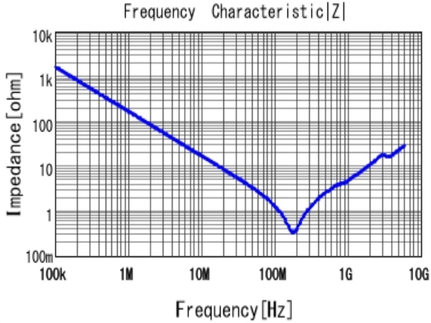
■ GRM31BR73A102KW01 |Z| DCOV, 25degC
