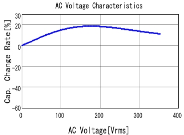
■ GRM31BR73A102KW01 C-AC Voltage capchange, DCOV, 25.0d
