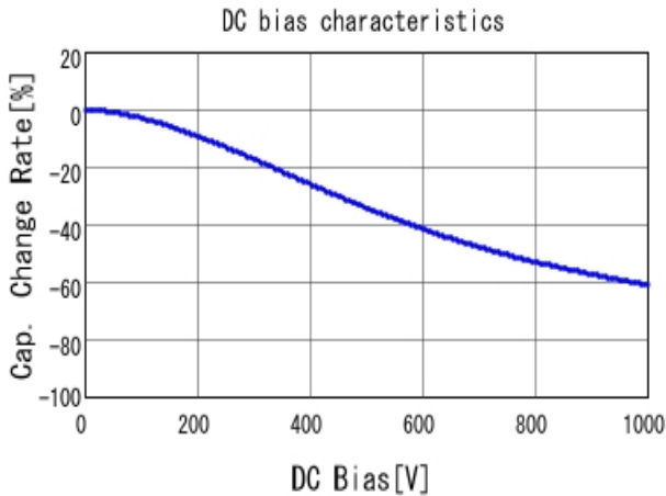
■ GRM31BR73A102KW01 C-DC bias capchange, 25.0degC, AC1V
