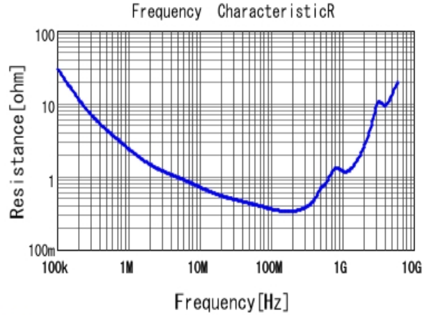
■ GRM31BR73A102KW01 R DCOV, 25degC
