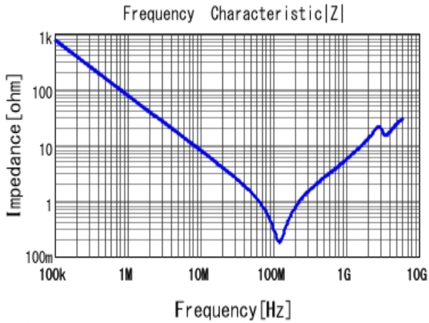
■ GRM31BR72J222KW01 |Z| DCOV, 25degC
