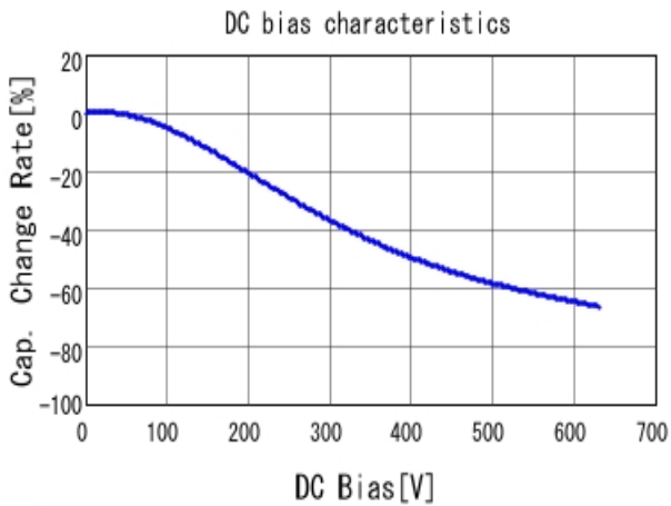
■ GRM31BR72J222KW01 C-DC bias capchange, 25.0degC, AC1V
