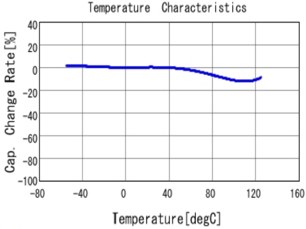
■ GRM31BR72J222KW01 C-Temp. capchange, DCOV, AC1Vrms
