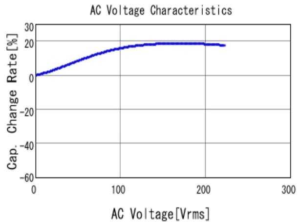
■ GRM31BR72J222KW01 C-AC Voltage capchange, DCOV, 25.0d
