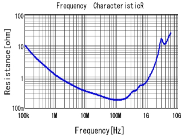
■ GRM31BR72J222KW01 R DCOV, 25degC
