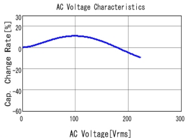
■ GRM31BR72J103KW01 C-AC Voltage capchange, DC0V, 25.0d
