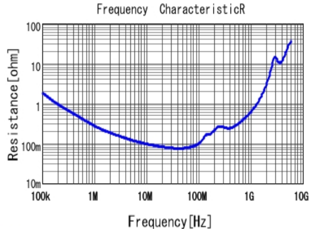
■ GRM31BR72J103KW01 R DC0V, 25degC
