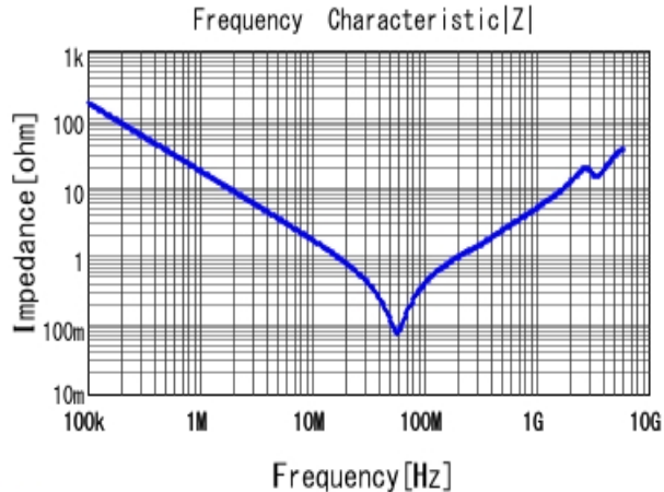
■ GRM31BR72J103KW01 |Z| DC0V, 25degC
