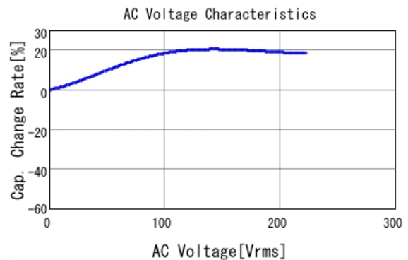
■ GRM31BR72J102KW01 C-AC Voltage capchange, DCOV, 25.0d
