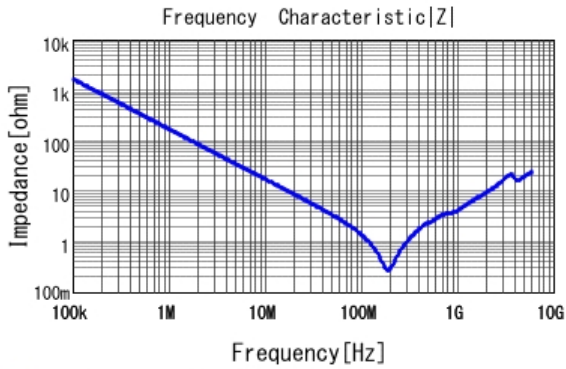
■ GRM31BR72J102KW01 |Z| DCOV, 25degC
