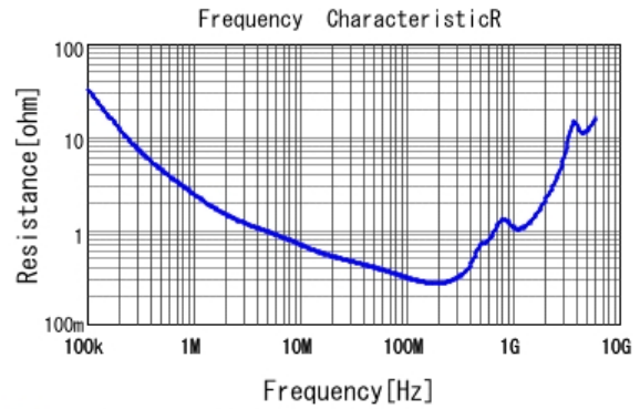
■ GRM31BR72J102KW01 R DCOV, 25degC
