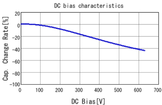
■ GRM31BR72J102KW01 C-DC bias capchange, 25.0degC, AC1V
