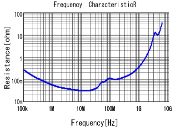
■ GRM31BR72E683KW01 R DCOV, 25degC
