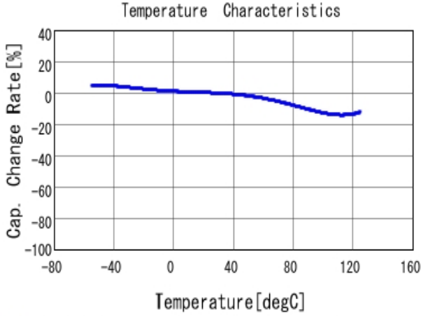
■ GRM31BR72E683KW01 C-Temp. capchange, DCOV, AC1Vrms
