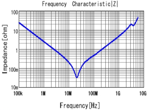
■ GRM31BR72E683KW01 |Z| DCOV, 25degC
