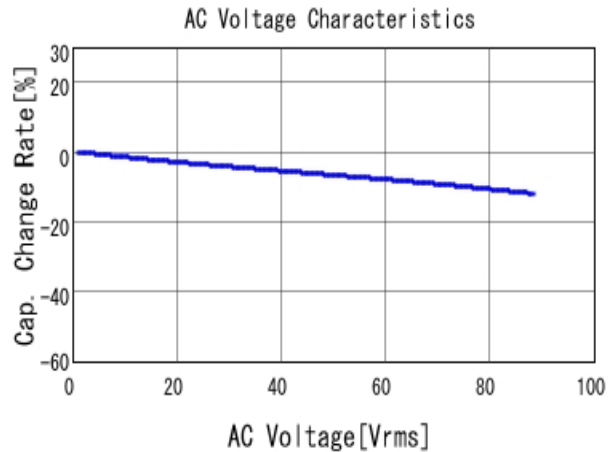
■ GRM31BR72E683KW01 C-AC Voltage capchange, DCOV, 25.0d
