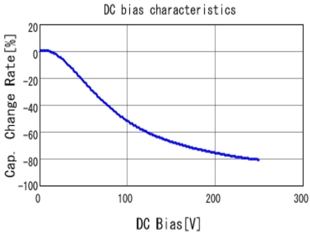
■ GRM31BR72E683KW01 C-DC bias capchange, 25.0degC, AC1V
