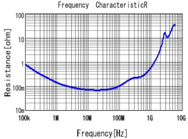
■ GRM31BR72E223KW01 R DCOV, 25degC
