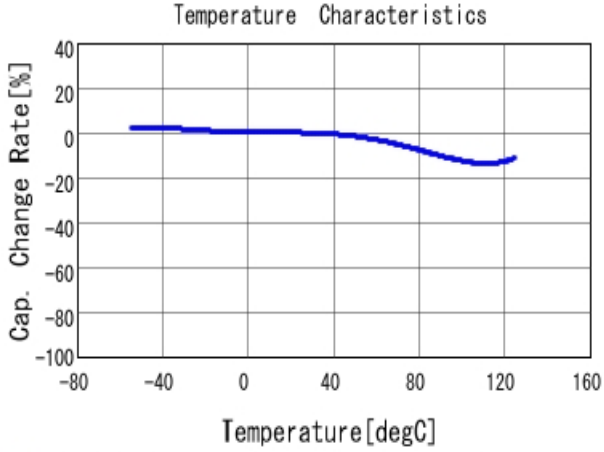
■ GRM31BR72E223KW01 C-Temp. capchange, DCOV, AC1Vrms
