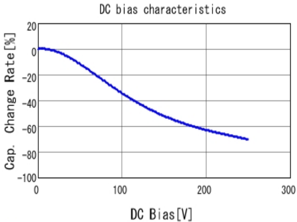
■ GRM31BR72E223KW01 C-DC bias capchange, 25.0degC, AC1V
