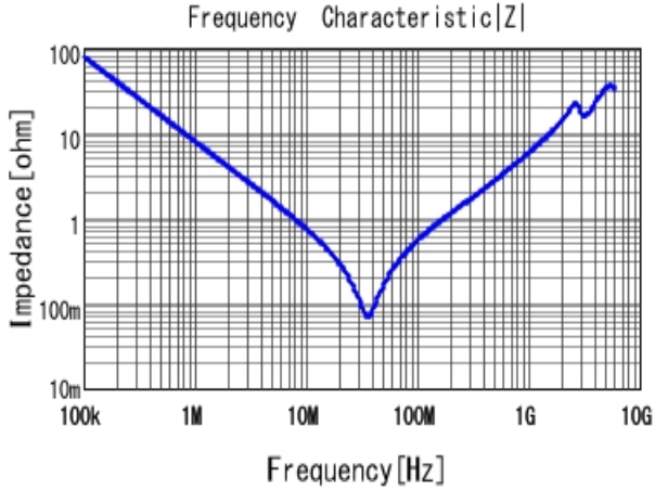
■ GRM31BR72E223KW01 |Z| DCOV, 25degC
