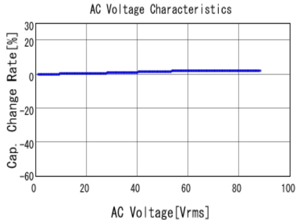
■ GRM31BR72E223KW01 C-AC Voltage capchange, DCOV, 25.0d
