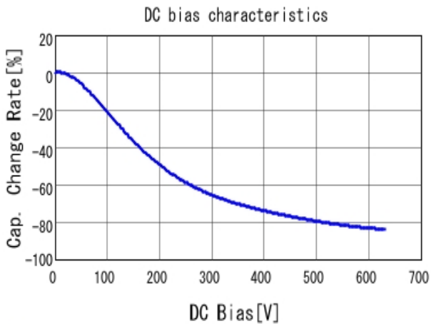
■ GRM31AR72J103KW01 C-DC bias capchange, 25.0degC, AC1V
