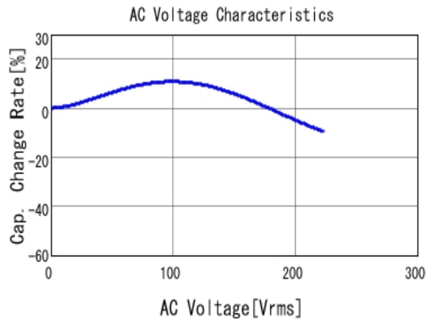
■ GRM31AR72J103KW01 C-AC Voltage capchange, DCOV, 25.0d
