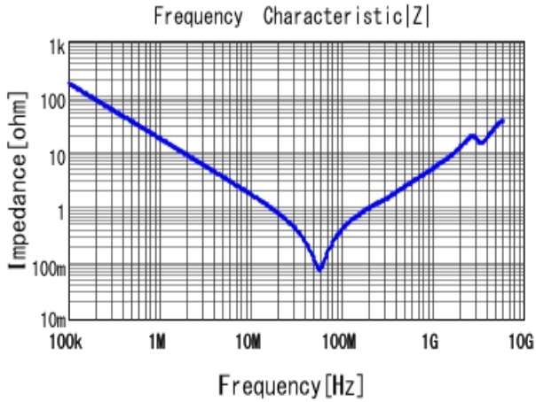
■ GRM31AR72J103KW01 |Z| DCOV, 25degC
