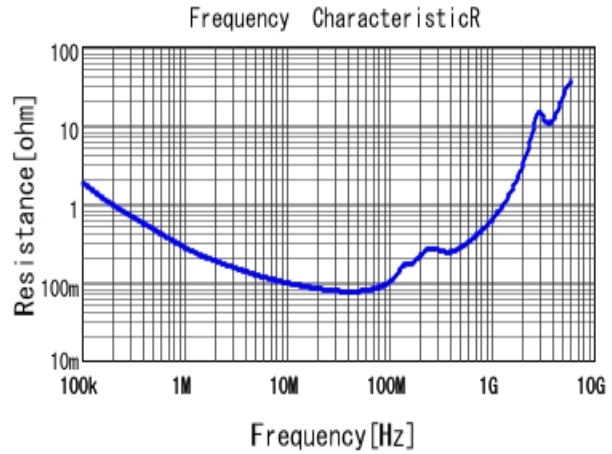
■ GRM31AR72J103KW01 R DCOV, 25degC
